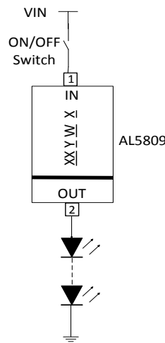
b) PWM Dimming by Power Supply VIN ON/OFF
