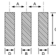
Figure 2) Land Pattern
