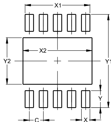
V-DFN3030-10 (Standard)
