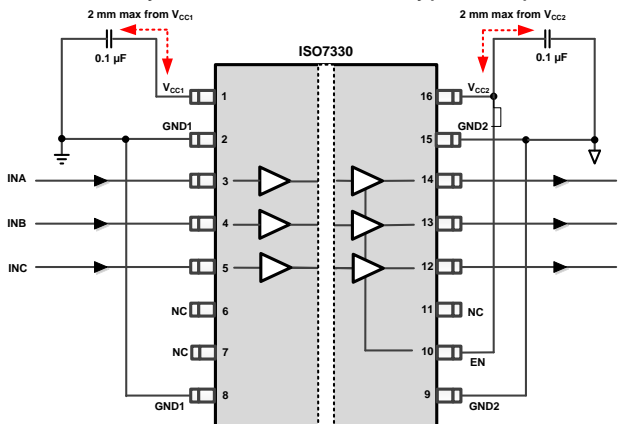
Figure 21. Typical ISO7330 Circuit Hook-up
