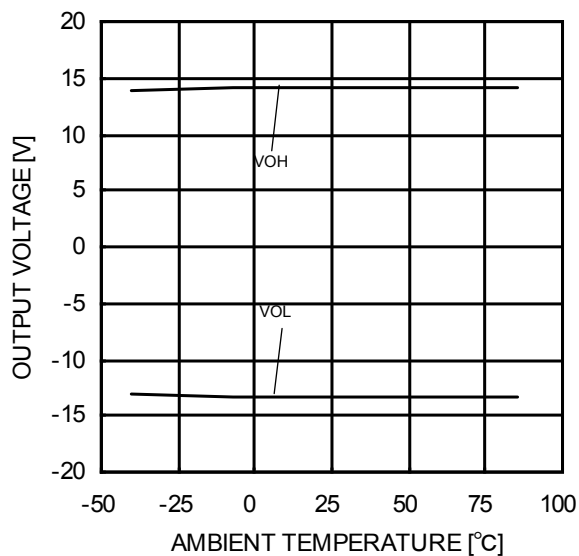
Figure 30. Maximum Output Voltage - Ambient Temperature (VCC/VEE=+15V/-15V, RL=2kΩ)
