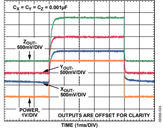
Figure 22. Typical Turn-On Time, V_S = 3V
