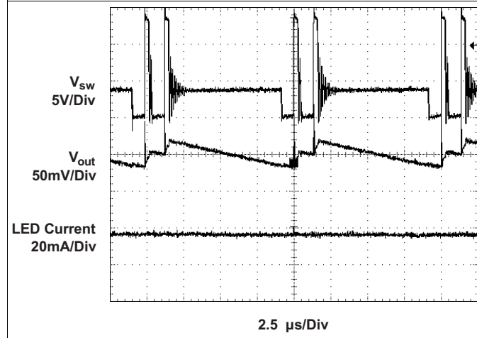
Figure 25. Bust Mode Operation
