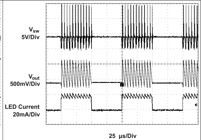
Figure 24. PFM Operation
