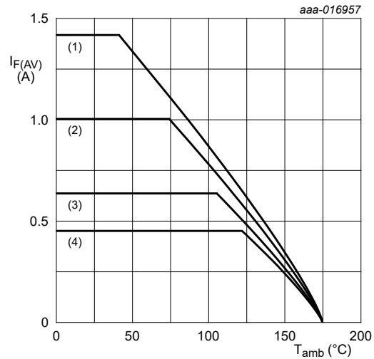
FR4 PCB, standard footprint T_j = 175 °C (1) \delta = 1 ; DC (2) \delta = 0.5 ; f = 20 kHz (3) \delta = 0.2 ; f = 20 kHz (4) \delta = 0.1 ; f = 20 kHz
