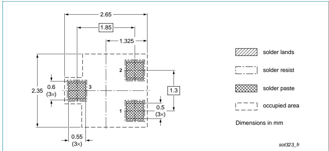
Fig 20. Reflow soldering footprint PDTC143EU (SOT323/SC-70)
