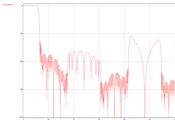
Figure 57 DAC Filter Response ( f_s=12\text{kHz} )
