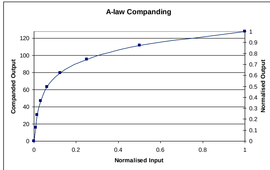
Figure 52 A-Law Companding
