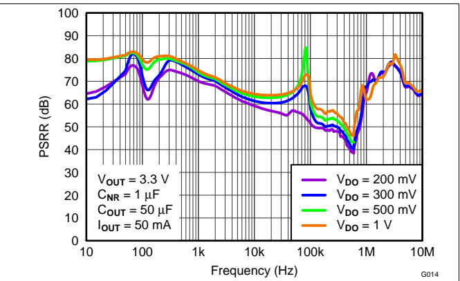
Figure 14. Power-Supply Rejection Ratio vs Dropout
