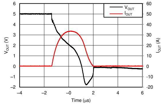
Figure 9-18. 50-mΩ Hot-Short Response Time
