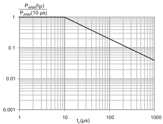
Figure 4. Normalized avalanche power derating versus pulse duration ( T_j = 125 \text{ }^\circ\text{C} )
