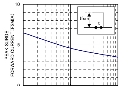
IFSM-t CHARACTERISTICS
