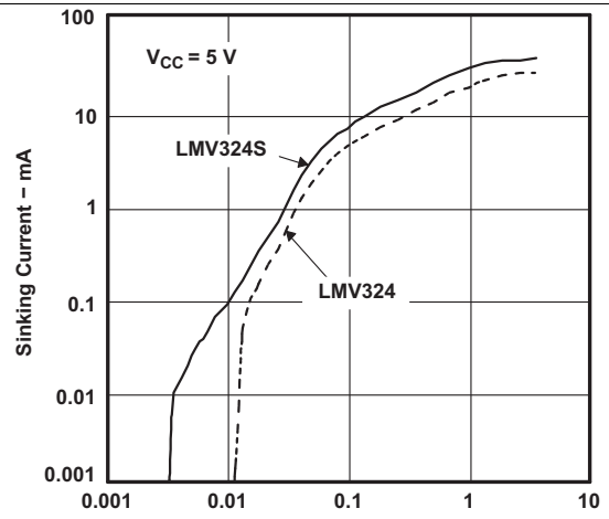
Figure 16. Sinking Current vs Output Voltage
