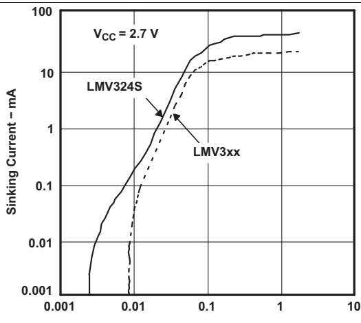
Figure 15. Sinking Current vs Output Voltage
