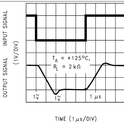
Figure 35. Noninverting Large Signal Pulse Response
