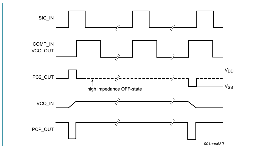
Fig 5. Typical waveforms for phase-locked loop with a locked phase comparator 2
