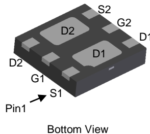
U-DFN2020-6 (Type B)
