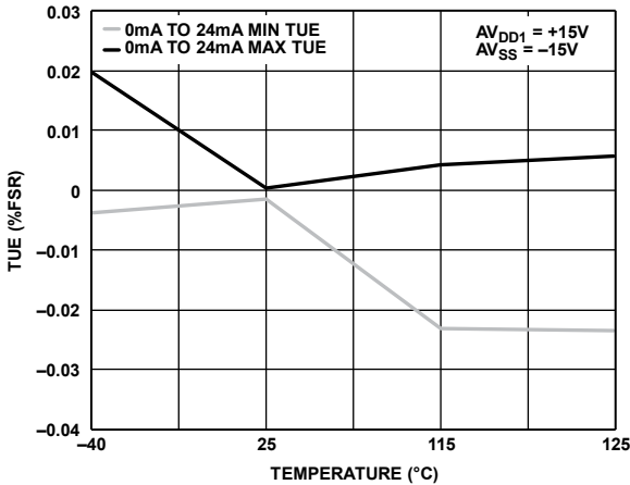
Figure 32. TUE vs. Temperature, External R_{SET}
